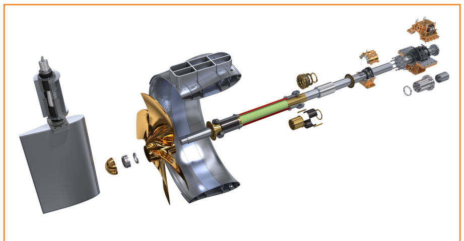
Example of water lubricated propeller shaft line.
