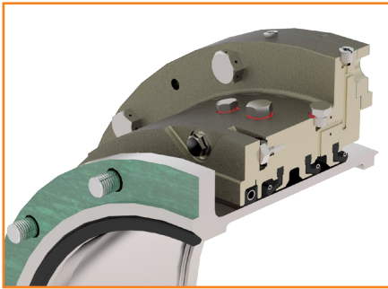
Example of air seal.
