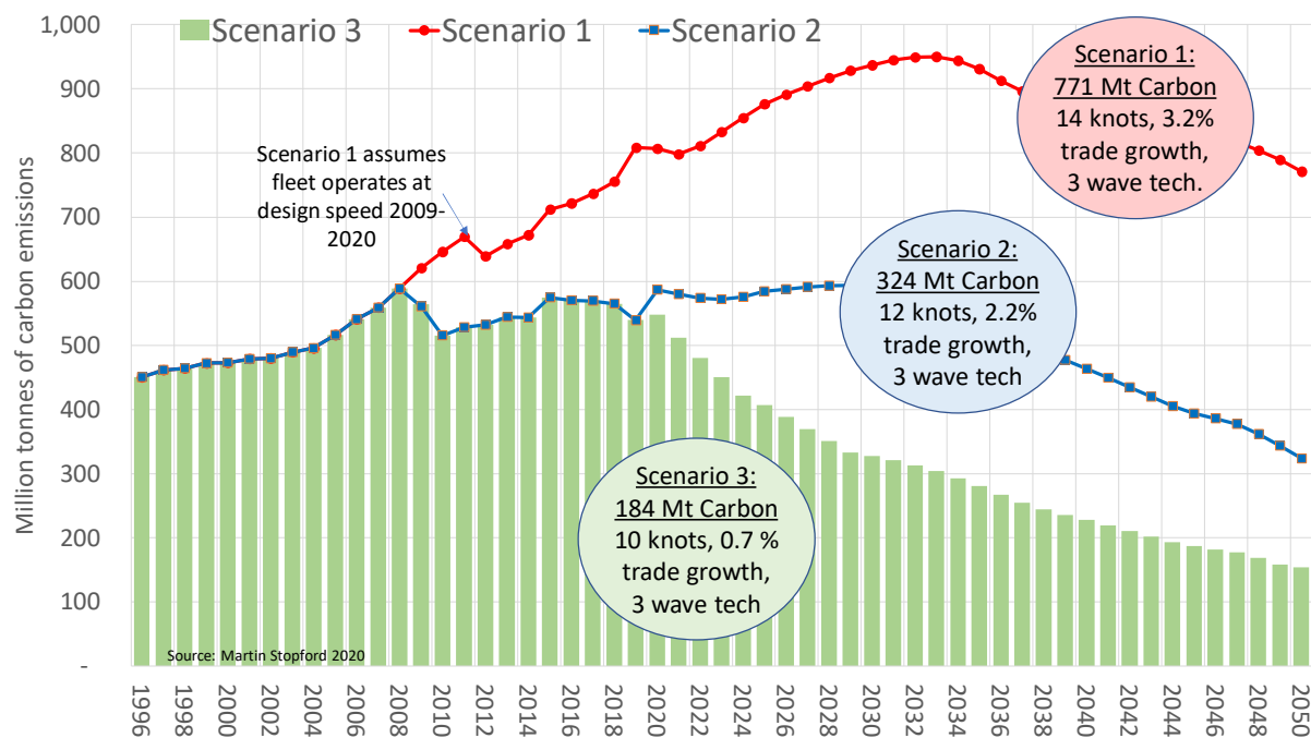
Figure 5 : Carbon emissions for scenarios 1-3 based on trade, shipbuilding & technical scenarios
